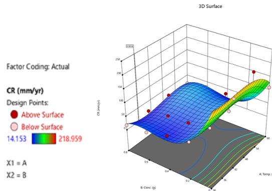
Figure 8: optimization Parameter plots of Chicken bone ash on copper
