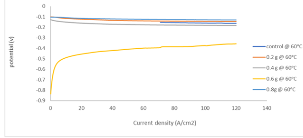
Figure 2: OCP graph for Chicken bone Inhibition @ 60°C
