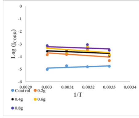
Figure 7: Temperature effect on copper corrosion in NaCl with and without the Chicken bone Inhibition
