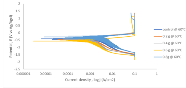
Figure 4: LSV Plot for Chicken bone Inhibition @ 60°C
