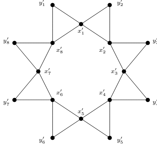
Figure 1: Schematic line graph L(S_n) of a sun-let graph S_n ( n = 8 shown)
