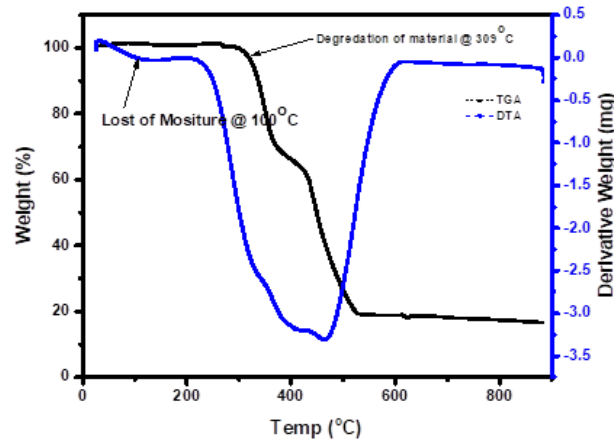
Figure 2: TGA and DTG profiles of Polyphenol-Rich Extract of S. Senegal (PRFSS)
