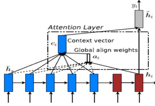
Figure 4: Information structure of Attention Mechanism
